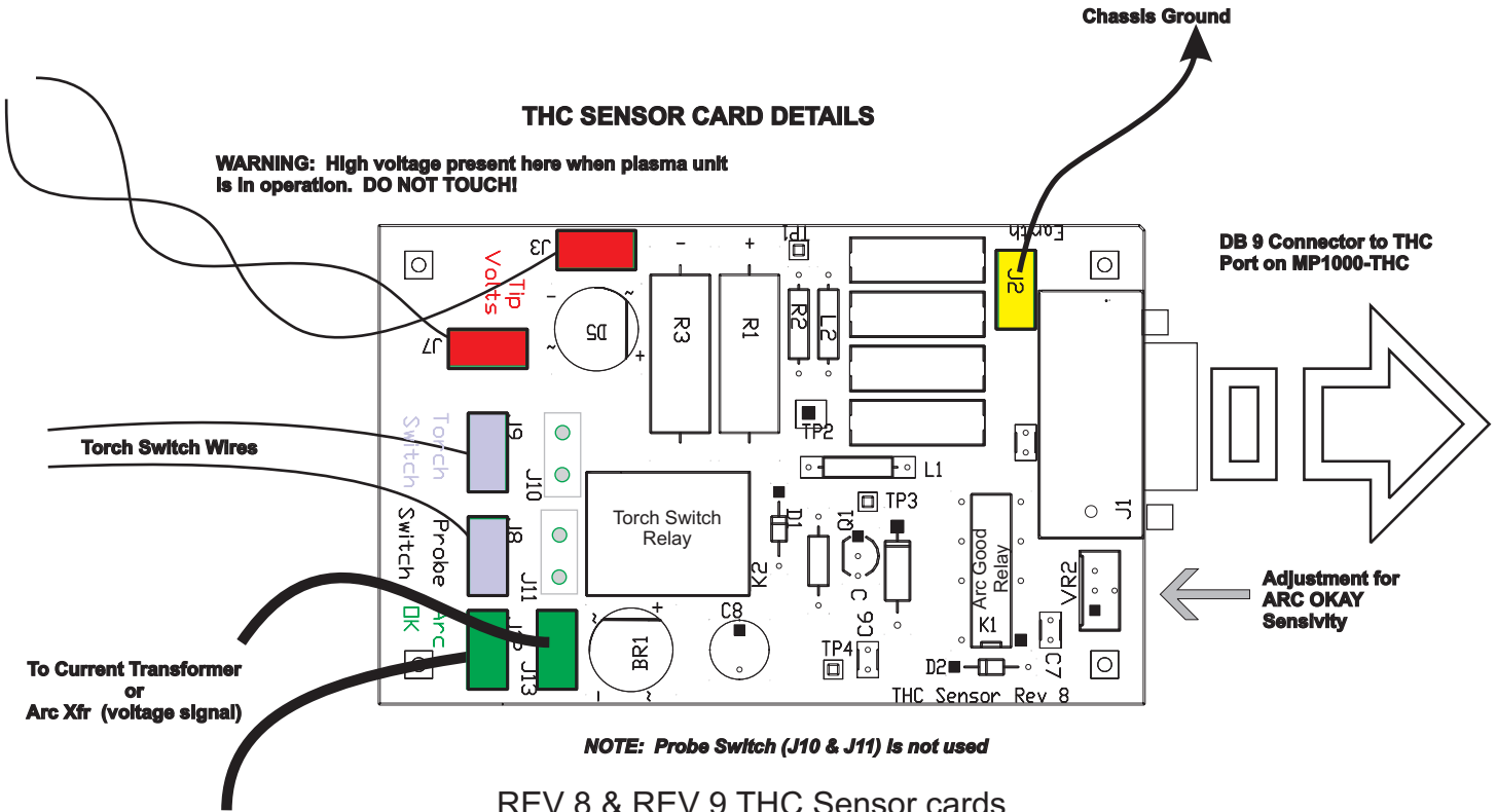
REV 8 & REV 9 THC Sensor cards
